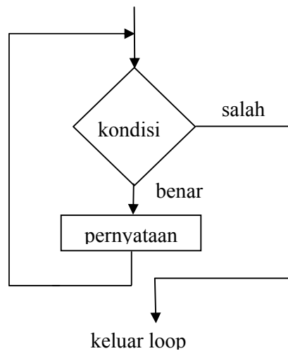
Gambar 4.2. Diagram alir while
